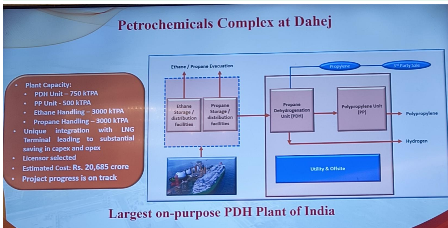
Exhibit 4: Flowchart of Petrochemical Complex
